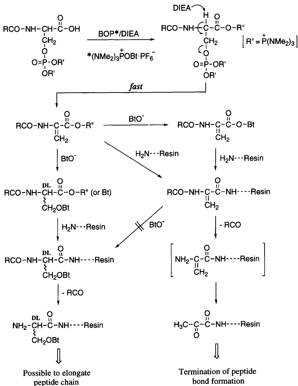
Figure 1. Plausible pathways of undesirable reactions occurring through the activation of O -(dialkyoxyphosphinyl)serine derivatives by the use of BOP for peptide bond formation.
